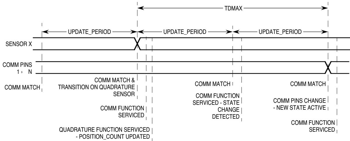
Figure 7 Sensorless Configuration
