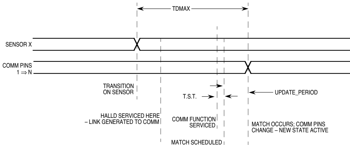
Figure 6 Sensorless Configuration
